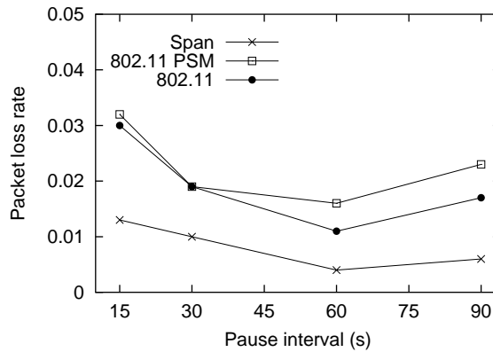
Figure 6: Packet loss rate as a function of pause time. The simulation area is a 1000 meter \times 1000 meter square. Mobility does not affect Span very much, and geographic forwarding with Span delivers more packets than with 802.11 PSM and 802.11 because it encounters fewer voids.
