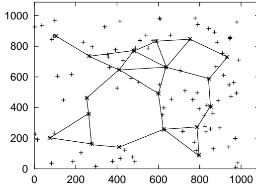
Figure 3: A scenario with 100 nodes, 19 coordinators, and a radio range of 250 meters. The nodes marked “*” are coordinators; the nodes marked “+” are non-coordinator nodes. Solid lines connect coordinators that are within radio range of each other.
