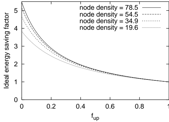
Figure 12: Energy savings as a function of f_{up} , computed using Equation 6, substituting C_{ideal} and 0.157 as values for C and \alpha . This figure shows that as f_{up} increases, the amount of energy saving decreases as well. In our experiments, f_{up} was between 0.185 and 0.263.
