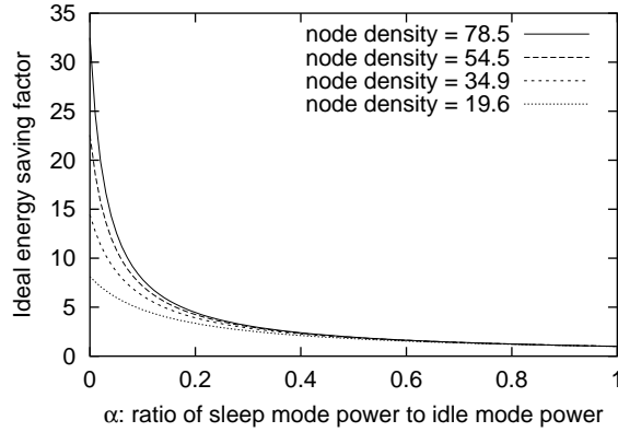
Figure 11: Energy savings as a function of \alpha , computed using Equation 6, substituting C_{ideal} and 0 as values for C and f_{up} when computing f_{idle} . This figure shows that as \alpha increases, the amount of energy saving decreases significantly. In our experiments, we used \alpha = 0.16 .
