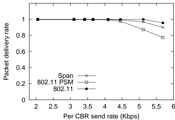
Figure 5: Packet delivery rate as a function of per-CBR-flow bit rate. Each packet traverses six hops. Under higher traffic load, Span delivers more packets than 802.11 PSM, but slightly less than 802.11.
