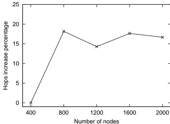
Figure 5: The percentage by which L^+ routes are longer than geographic shortest paths, as a function of total number of nodes in the network.
