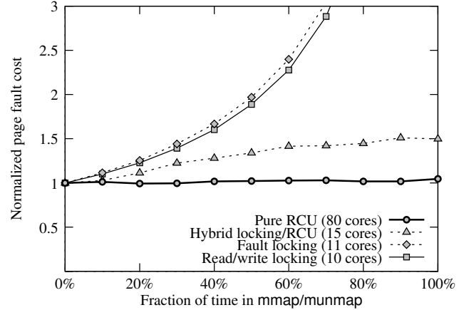
Figure 18. Microbenchmark page fault cost with varying time spent in mmap and munmap , shown relative to the cost with no concurrent memory mapping operations.
