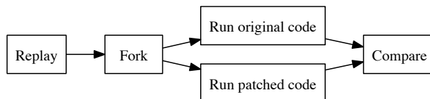
Figure 1: The workflow of retroactive auditing.
