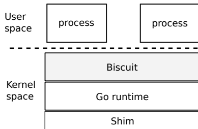
Figure 1: Biscuit’s overall structure.
